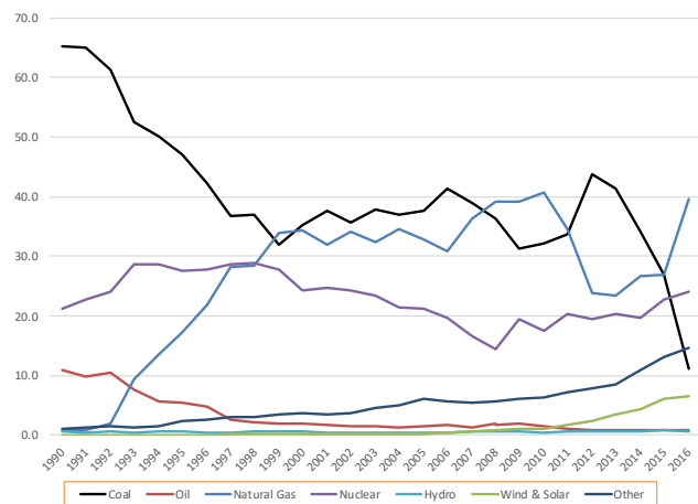
Figure 2: Fuel Input for Power Generation Source: BEIS (2017a)
